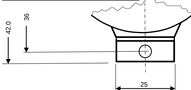
SCRAP VIEW SHOWING VFLx CONNECTION
